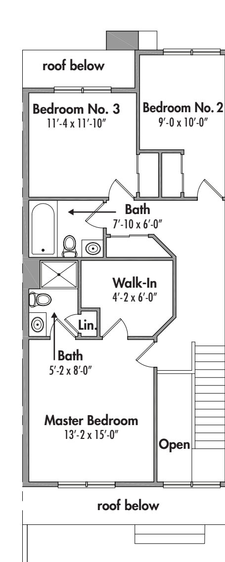
Second Floor
